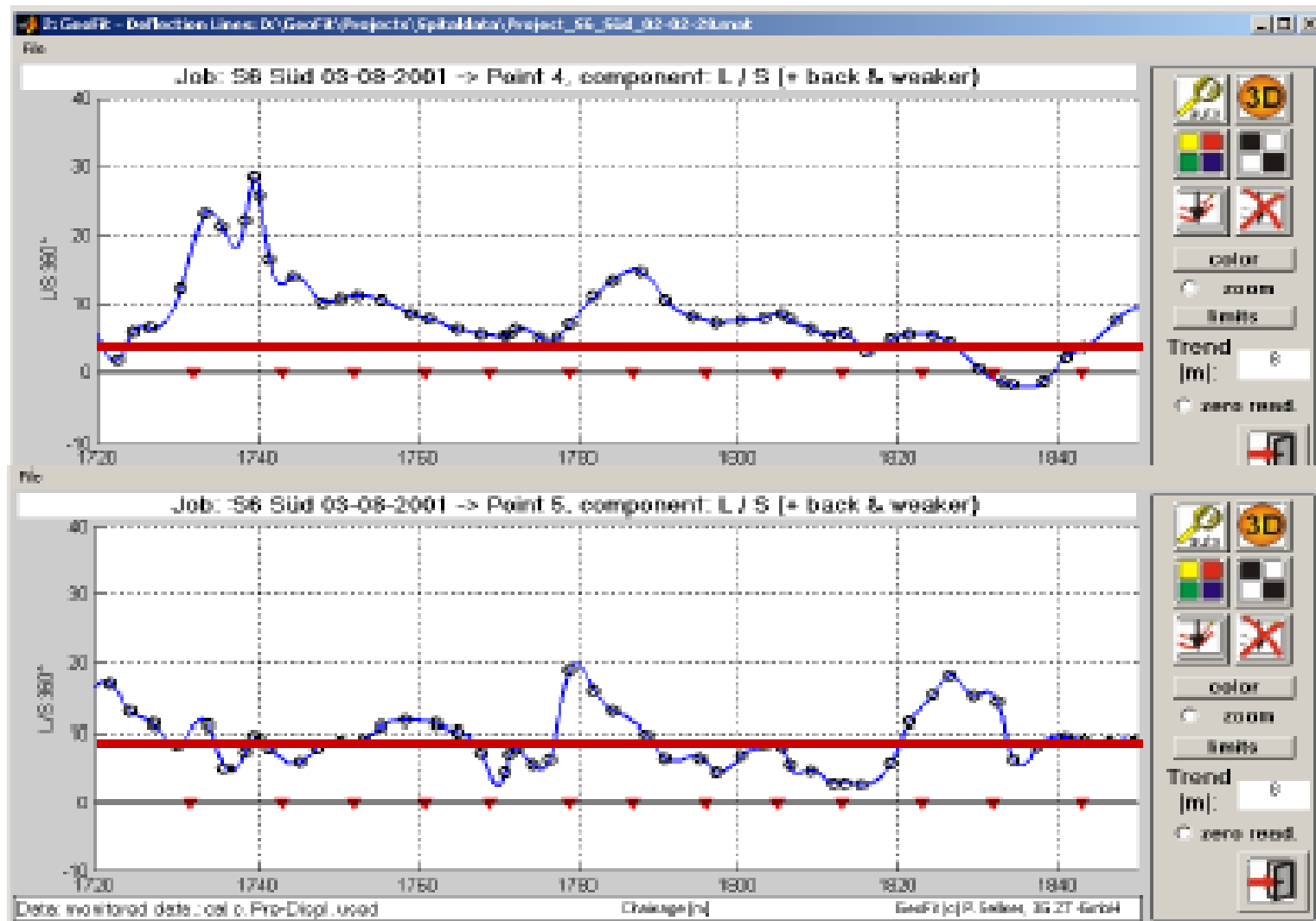
Figure 10. Comparison of the vector orientation plots for points 4 and 5 between stations 1720 and 1850. The “normal” orientation is approximately 8°-10°. The trend is developed 8 m behind the tunnel face.
